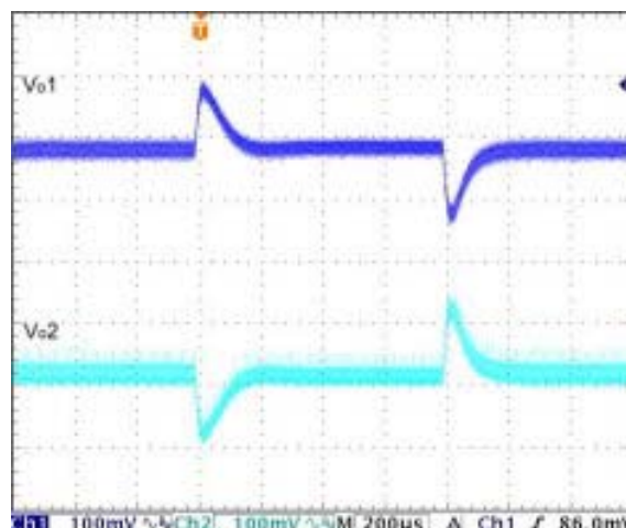
Graph 8: Transient Response to Dynamic Load Change from 100% to 75% to 100% of Full Load at Nominal Vin
