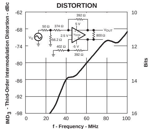
THIRD-ORDER INTERMODULATION DISTORTION
