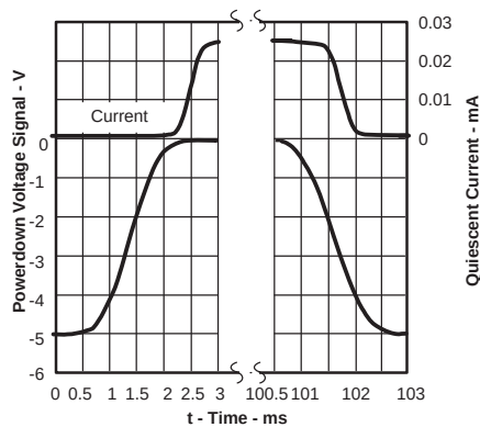
TURNON AND TUNOFF DELAY TIMES
