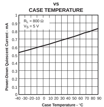
POWER-DOWN QUIESCENT CURRENT
