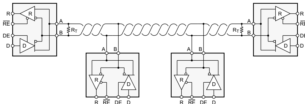
Simplified Schematic
