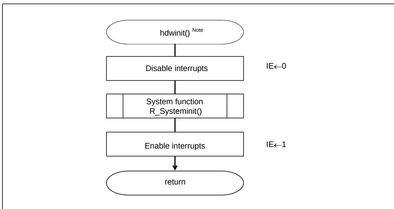
Figure 5.2 Initialization Function
