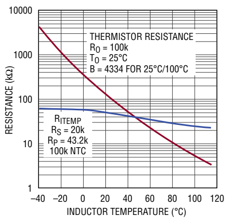
Figure 5. Resistance Versus Temperature for the ITEMP Pin Network and the 100k NTC
