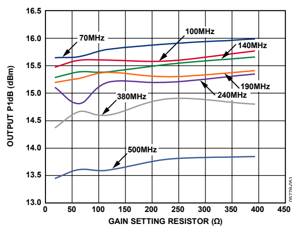
Figure 13. Output 1 dB Compression Point vs. R_G for Multiple Frequencies, R_L = 200\ \Omega
