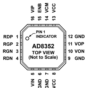
Figure 3. Pin Configuration
