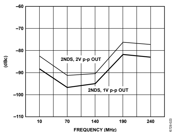
Figure 30. Single-Ended, Second-Order Harmonic Distortion, 1 kΩ Load
