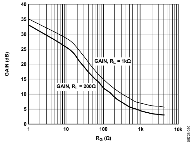
Figure 27. Gain vs. R_G
