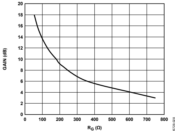
Figure 24. Gain vs. R_G , R_L = 1 \text{ k}\Omega
