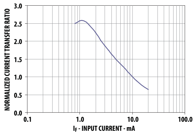
Figure 2. Current Transfer Ratio vs. Input Current V_0 = 0.4 V, V_{CC} = 5 V, T_A = 25^\circ C
