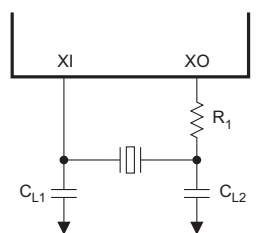
Figure 7-2. Crystal Oscillator Circuit
