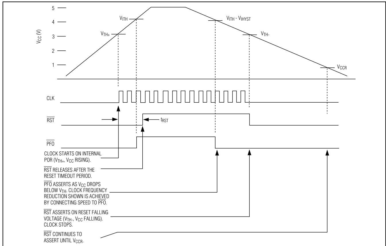
Figure 1. RST/\overline{RST} and \overline{PFO} Behavior During Power-Up and Brownout
