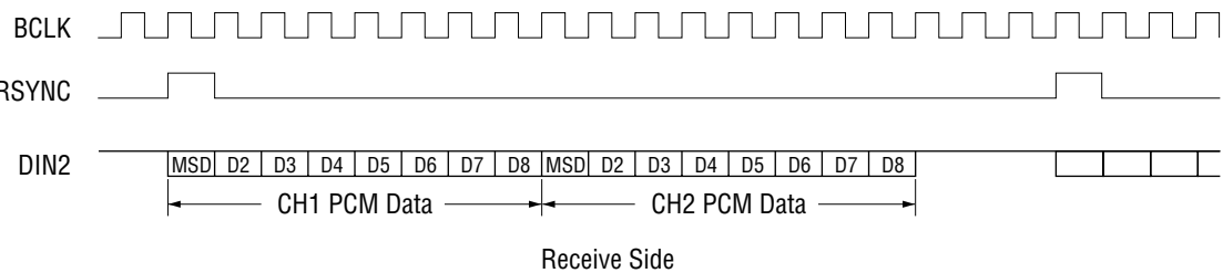
Figure 2 Timing Diagram in the Serial Mode (CHPS = 0)
