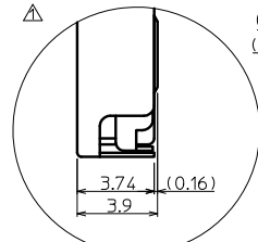
DETAIL B (5:1)
