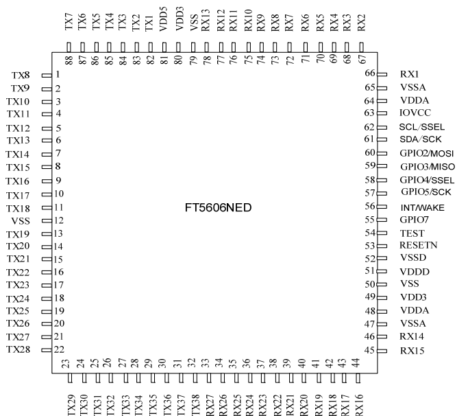
FT5606NED Package Diagram
