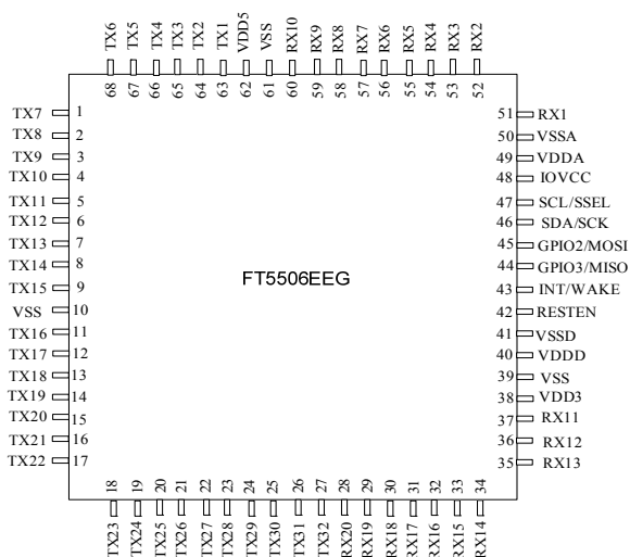
FT5506EEG Package Diagram
