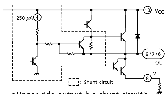
&lt;Upper side output b-e shunt circuit&gt;
