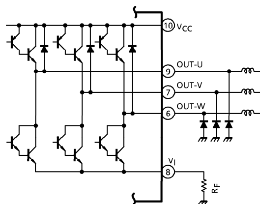
<Output circuit>
