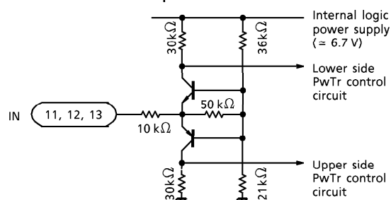
<Input circuit>
