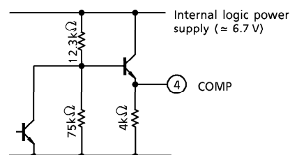
&lt;Output voltage detection circuit&gt;
