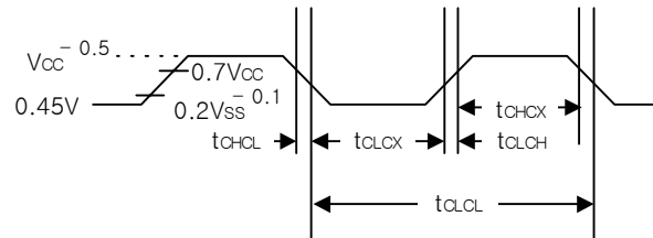
Figure 10. Clock Signal Waveform for I_{CC} Tests in Active and Idle Modes t_{CLCH} = t_{CHCL} = 5\text{ns}
