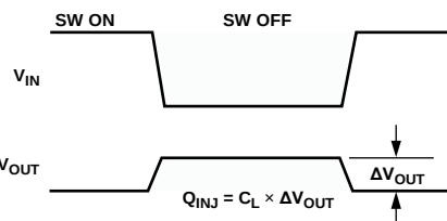
Figure 21. Charge Injection
