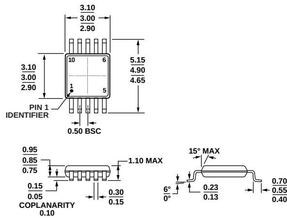
COMPLIANT TO JEDEC STANDARDS MO-187-BA Figure 25. 10-Lead Mini Small Outline Package [MSOP] (RM-10) Dimensions shown in millimeters
