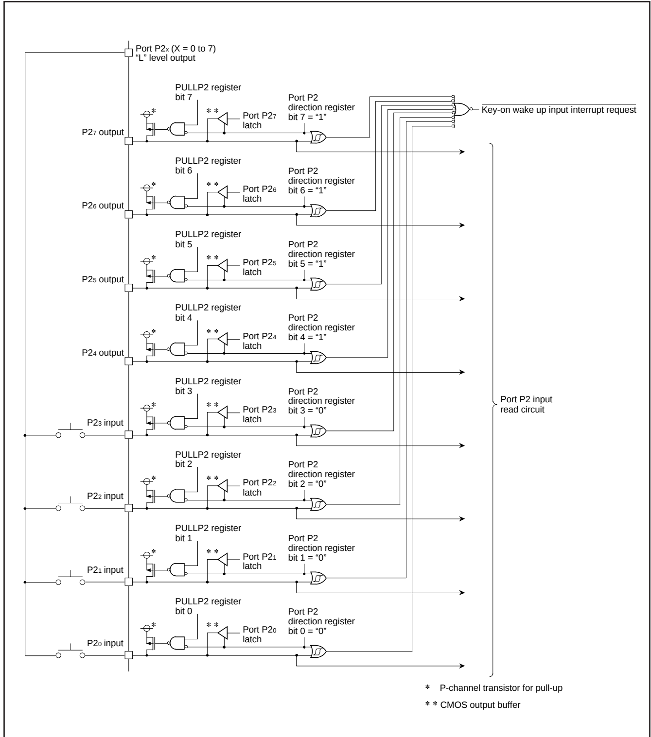
Fig. 25 Block diagram of port P2, and example of wired at used key-on wake up
