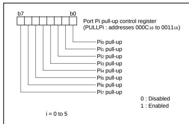
Fig. 4 Structure of port Pi pull-up control register
