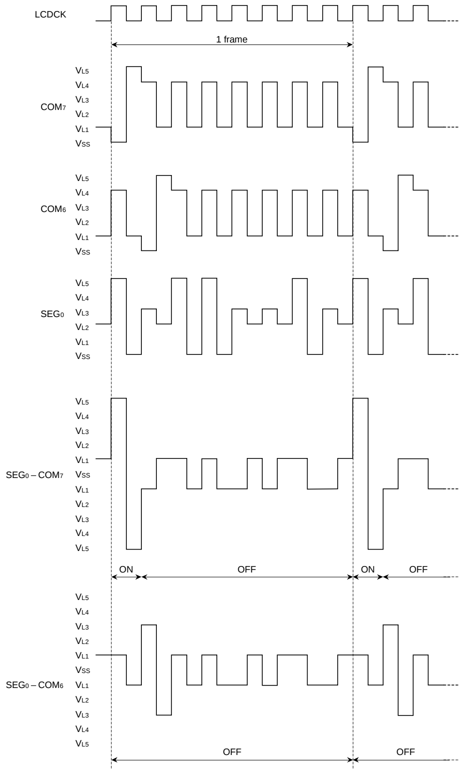
Fig. 23 1/8 duty, 1/5 bias, type-A LCD wave diagram
