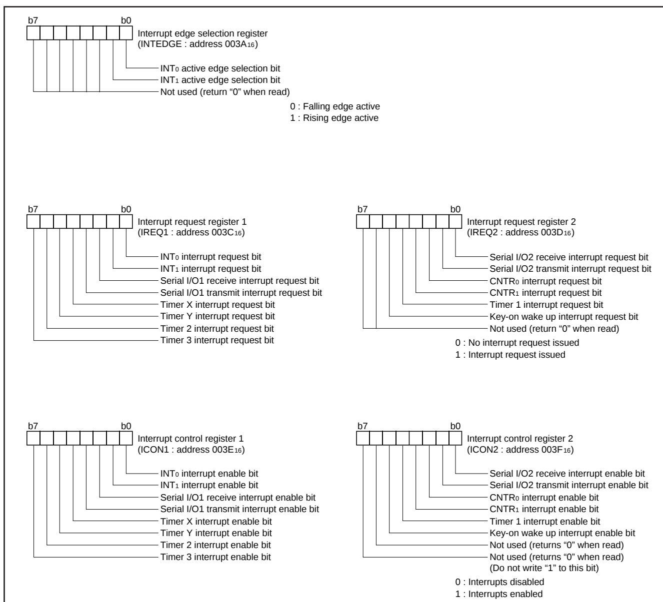
Fig. 8 Structure of interrupt-related registers
