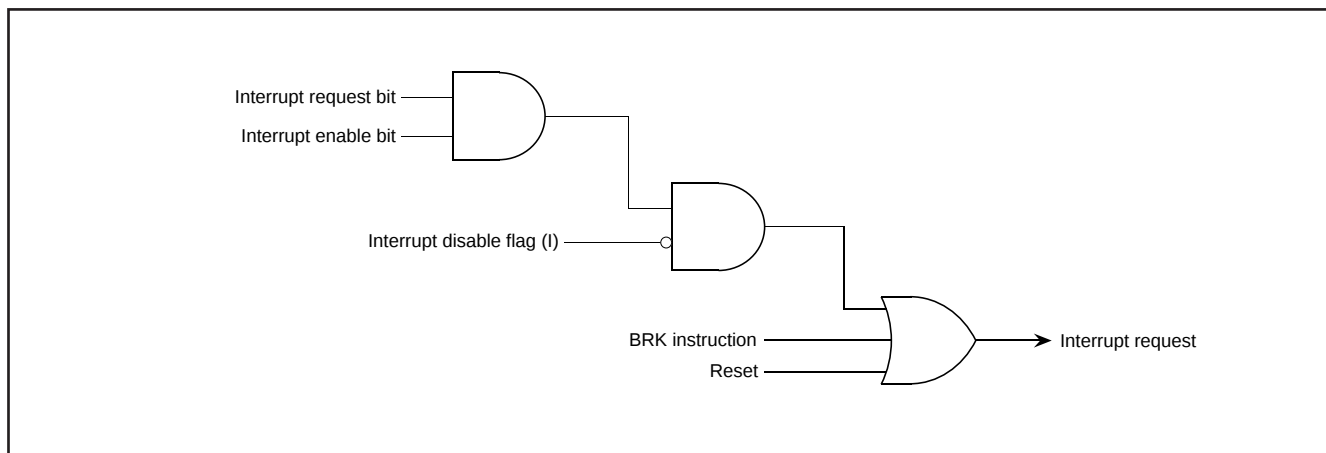
Fig. 7 Interrupt control
