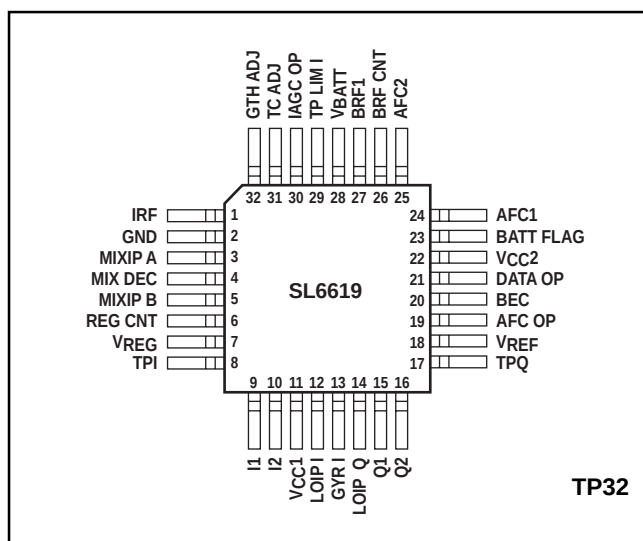
Fig. 1 Pin identification diagram (top view). See Table 1 for pin descriptions
