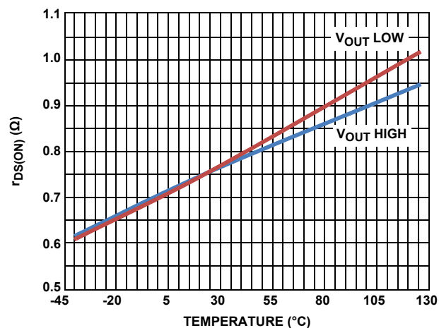
FIGURE 14. r_{DS(ON)} vs TEMPERATURE
