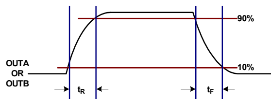
FIGURE 5. RISE/FALL TIMES
