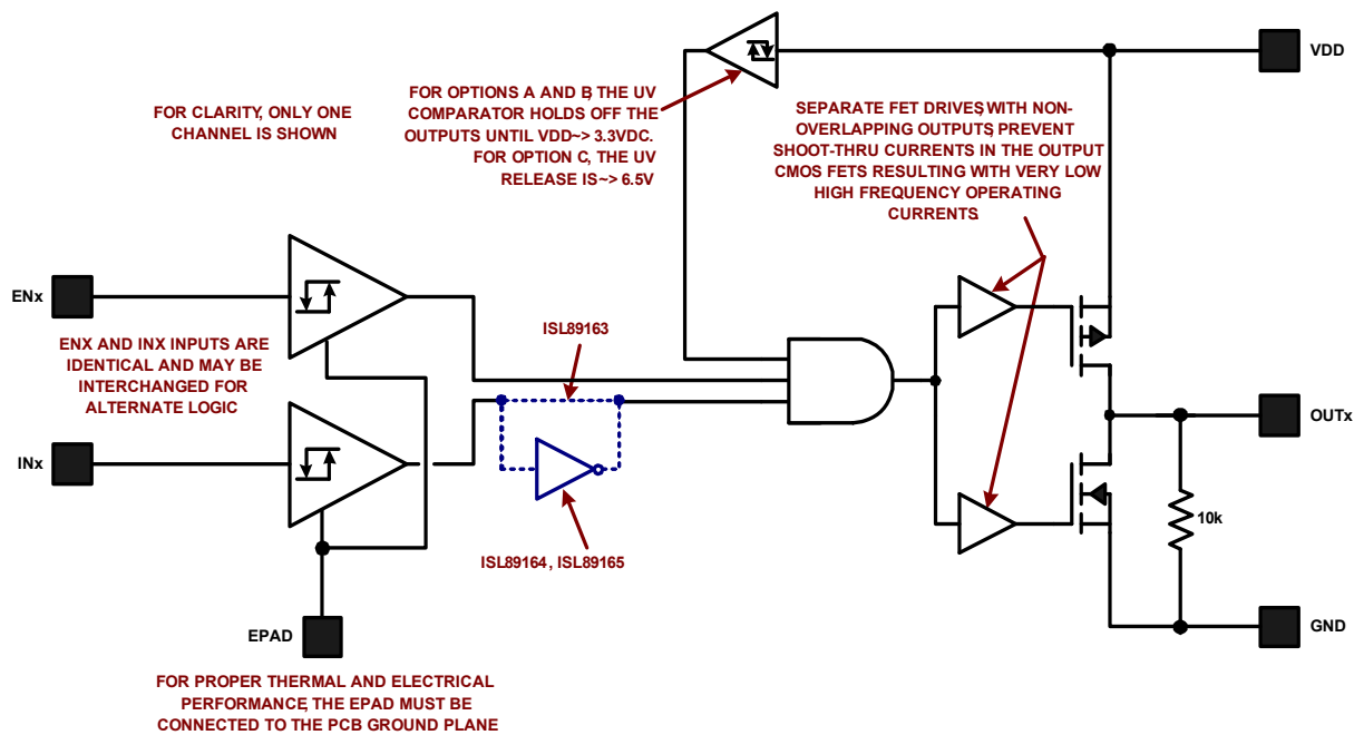
FIGURE 3. BLOCK DIAGRAM
