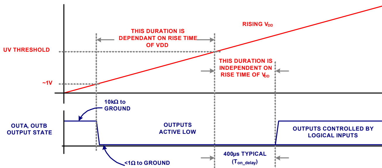
FIGURE 10. START-UP OUTPUT CHARACTERISTIC
