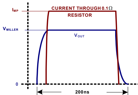
FIGURE 9. MILLER PLATEAU SOURCE CURRENT
