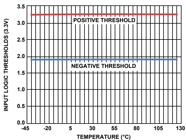
FIGURE 16. OPTION B THRESHOLDS
