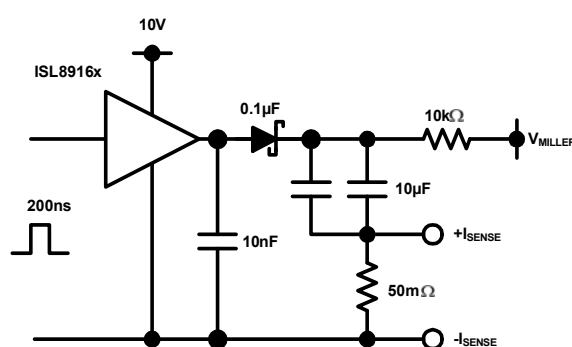
FIGURE 7. MILLER PLATEAU SOURCE CURRENT TEST CIRCUIT
