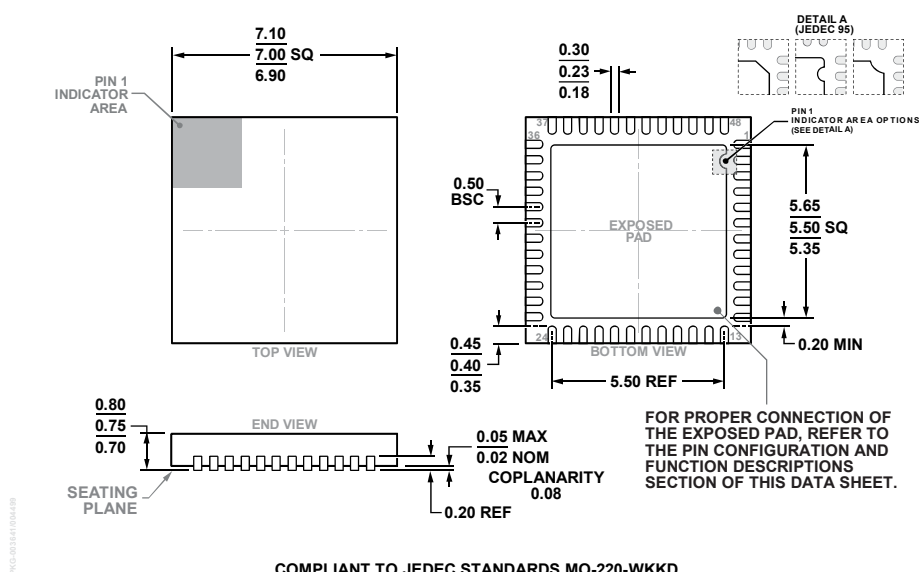
Figure 82. 48-Lead Lead Frame Chip Scale Package [LFCSP] 7 mm × 7 mm Body and 0.75 mm Package Height (CP-48-9)
