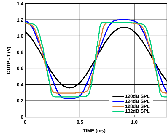
Figure 8. Clipping Characteristics
