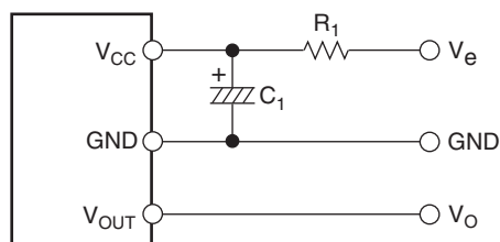
Fig. 5. Device Connection
