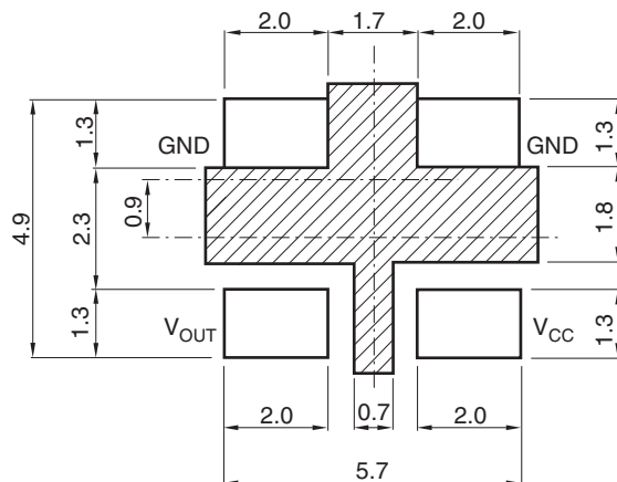
Fig. 7. Soldering Mask
