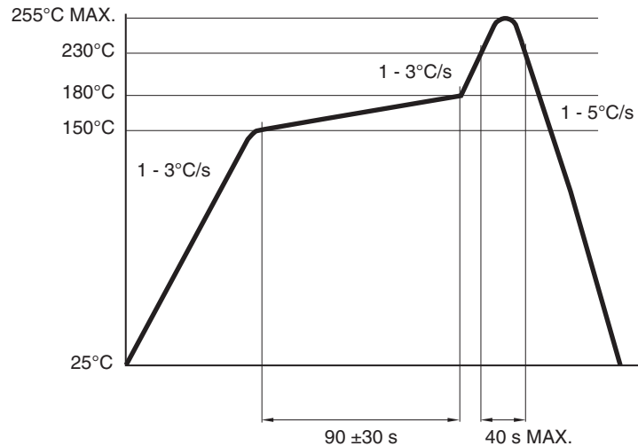
Fig. 6. Soldering Profile
