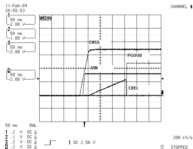
FIGURE 11. PGOOD DELAY
