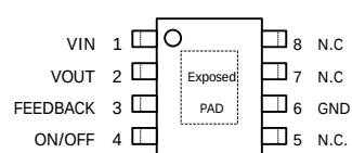
SOP8-PP
