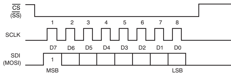
Figure 31. Interface Timing — Control Byte 1
