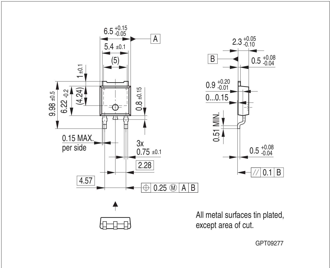
Figure 5 PG-TO252-3
