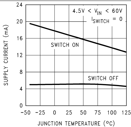
Figure 7. Quiescent Current
