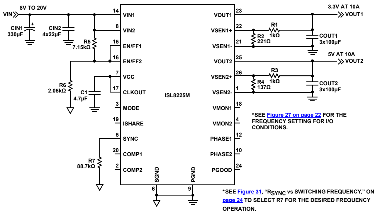
FIGURE 21. 3.3V/5V VOLTAGE APPLICATION WITH THE FREQUENCY SET AT 900kHz
