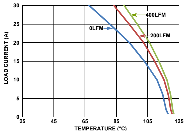
FIGURE 39. DERATING CURVE 5V TO 1.5V
