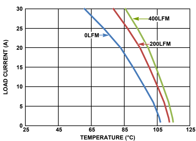
FIGURE 40. DERATING CURVE 12V TO 1.5V
