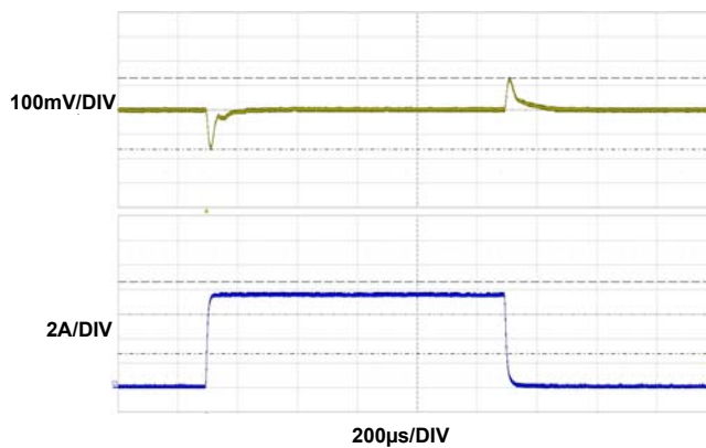
FIGURE 13. 3.3V OUT TRANSIENT RESPONSE
