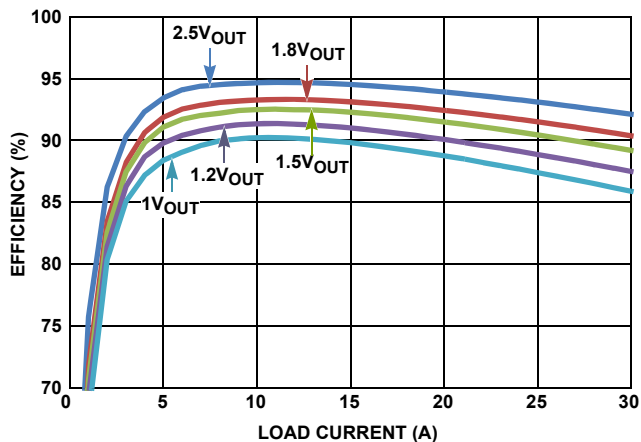
FIGURE 6. EFFICIENCY vs LOAD CURRENT (PARALLEL SINGLE OUTPUT, AS SHOWN IN Figure 19 AT 5V_{\text{IN}} /500kHz)
