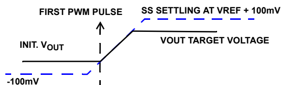
FIGURE 30. SOFT-START WITH V_{OUT} < \text{TARGET VOLTAGE}
