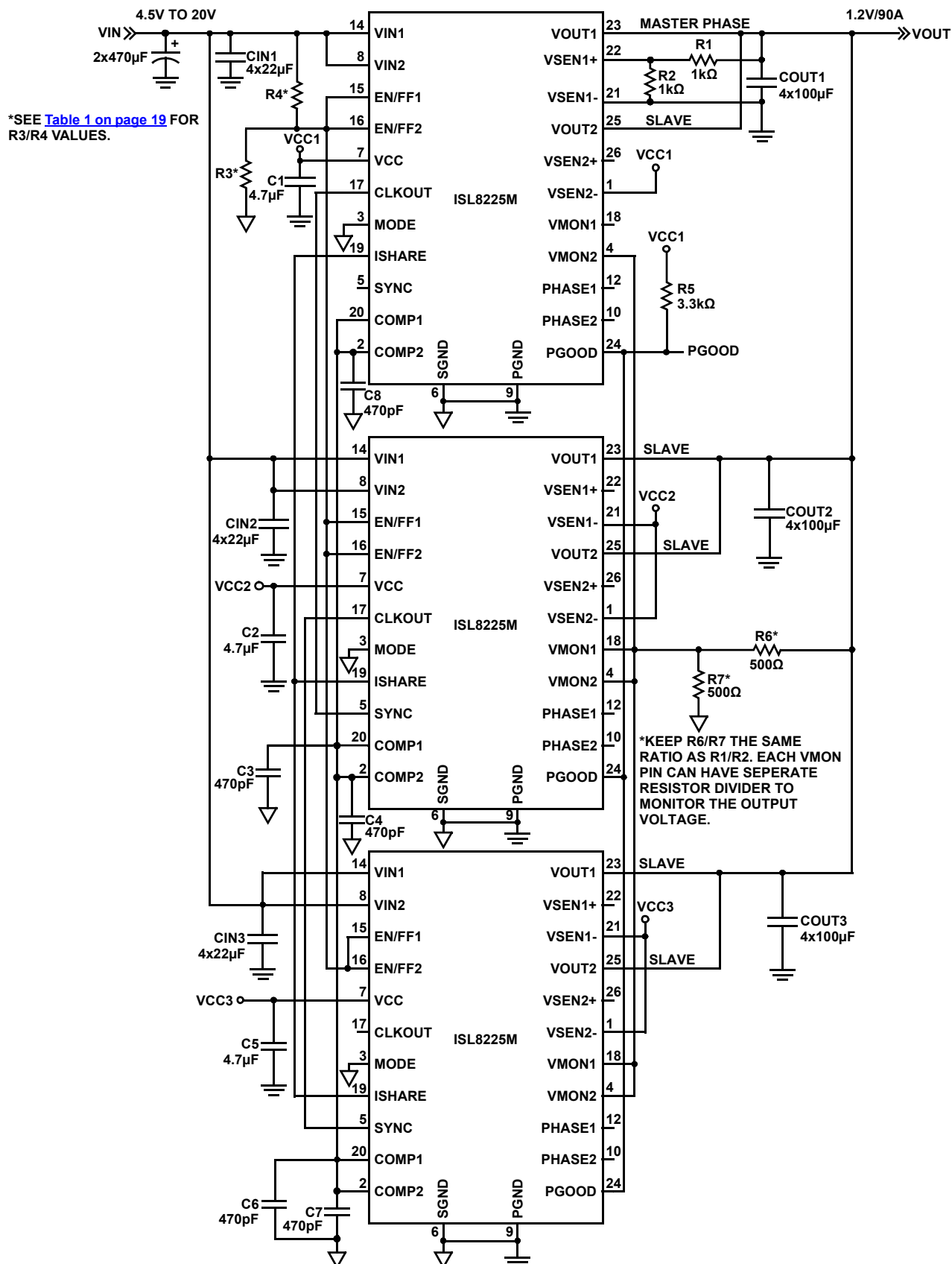
FIGURE 26. SIX-PHASE 90A 1.2V OUTPUT CIRCUIT
