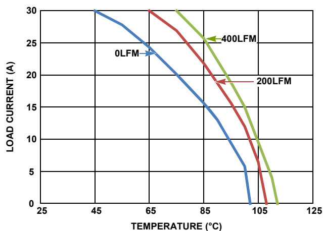
FIGURE 44. DERATING CURVE 12V/3.3V
