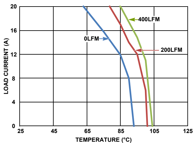
FIGURE 46. DERATING CURVE 12V/6.5V
