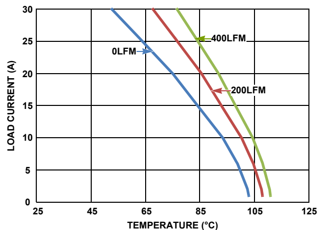
FIGURE 42. DERATING CURVE 12V TO 2.5V
