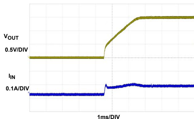
FIGURE 14. START-UP AT 0A
