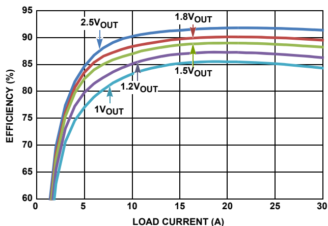
FIGURE 7. EFFICIENCY vs LOAD CURRENT (PARALLEL SINGLE OUTPUT, AS SHOWN IN Figure 19 AT 12V_{\text{IN}} /500kHz)
