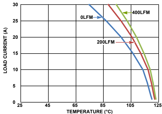
FIGURE 37. DERATING CURVE 5V TO 1V
