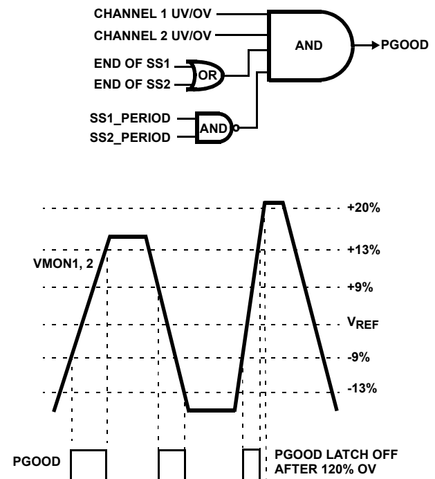
FIGURE 32. POWER-GOOD THRESHOLD WINDOW
