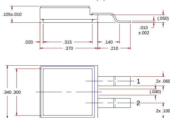
CerPack (G)
