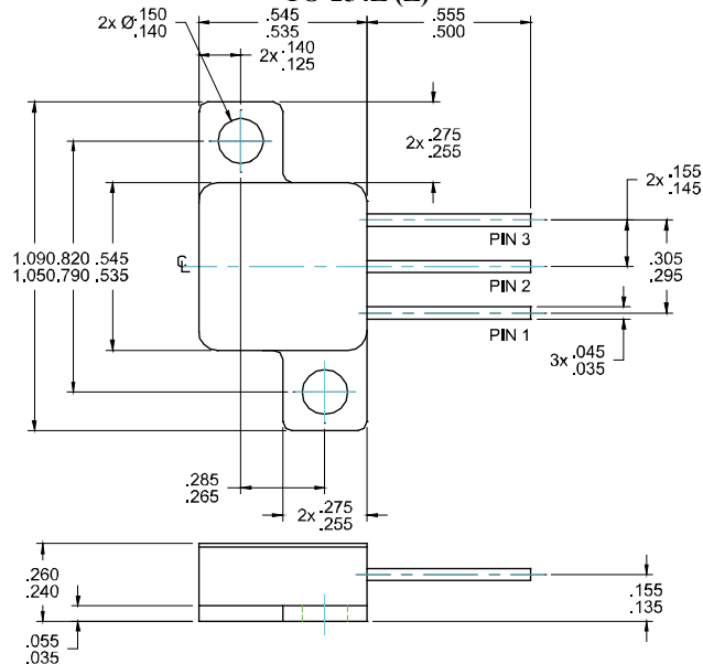
TO-254Z (Z)
