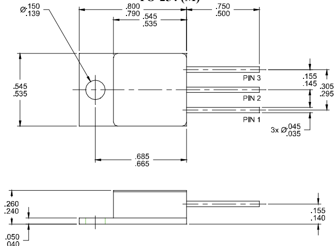
TO-254 (M)
