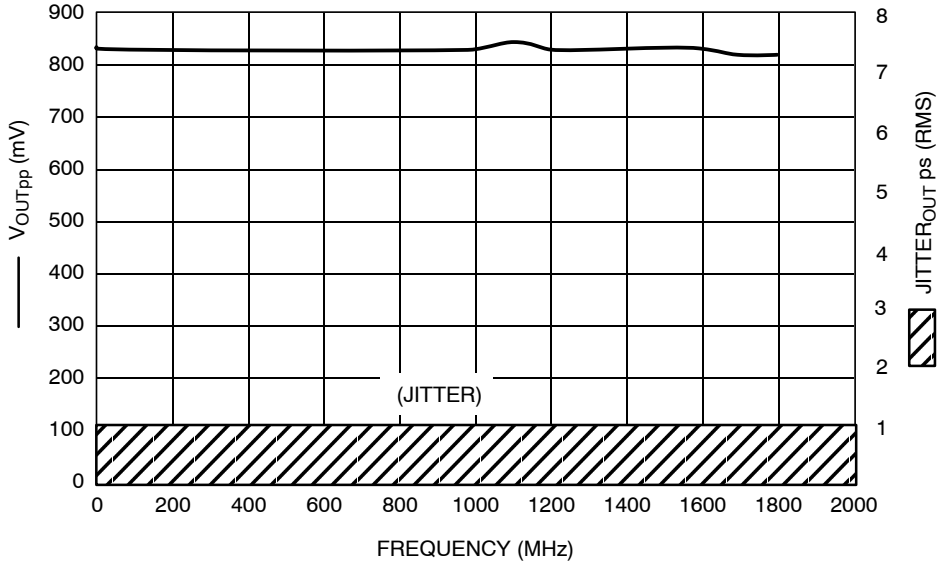
Figure 7. \div 5 , F_{max}/Jitter
