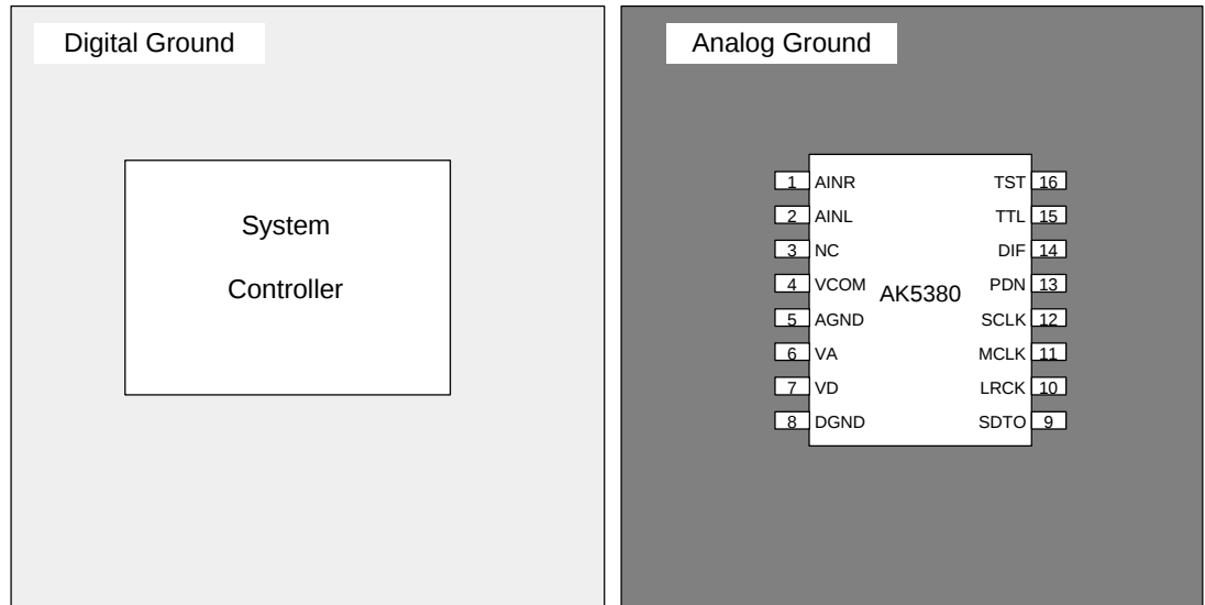
Figure 7. Ground Layout
