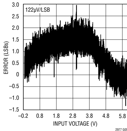
ADC-INL
