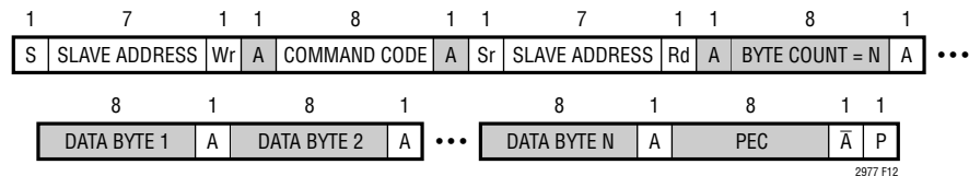
Figure 12. Block Read with PEC
