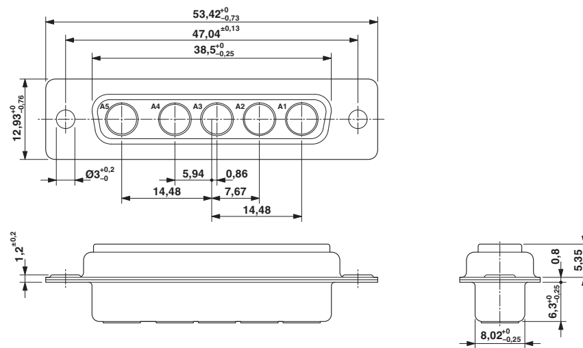
Dimensioned drawing
