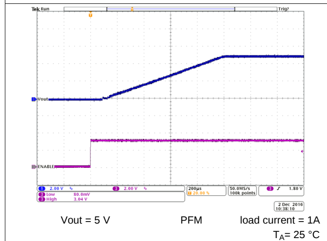
Figure 56. Start-Up Timing
