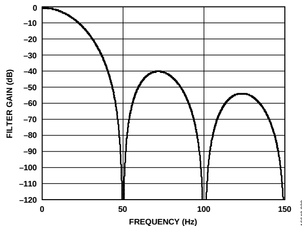
Figure 43. Sinc3 Filter Response
