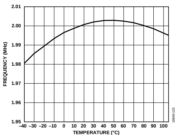
Figure 22. Internal Oscillator Frequency vs. Temperature
