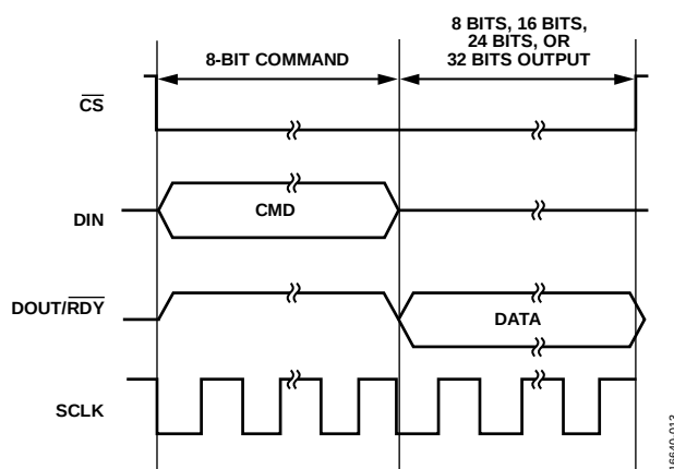
Figure 34. Reading from a Register (8-Bit Command with Register Address Followed by Data of 8 Bits, 16 Bits, 24, or 32 Bits; Data Length on DOUT Is Dependent on the Register Selected)
