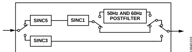
Figure 41. Digital Filter Block Diagram
