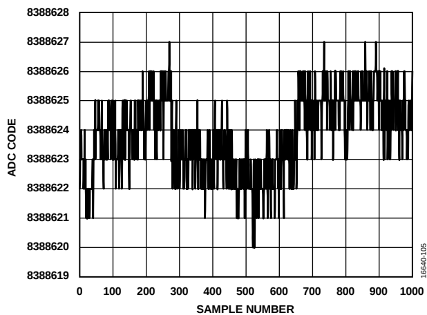
Figure 5. Noise (Voltage Input, Output Data Rate = 1.25 SPS)
