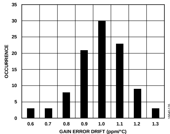
Figure 26. Gain Error Drift Distribution Histogram (Voltage Input)
