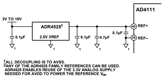
Figure 39. ADR4525 Connected to AD4111 REF± Pins
