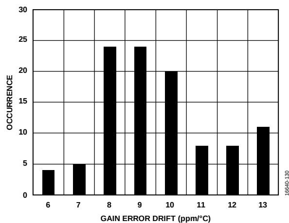
Figure 30. Gain Error Drift Distribution Histogram (Current Input)
