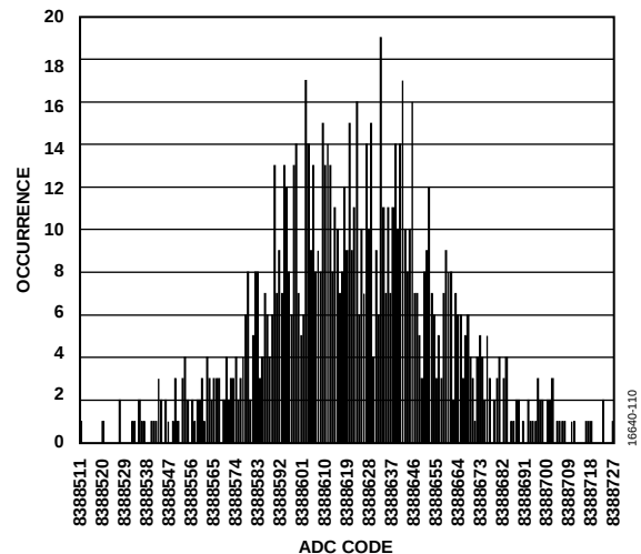
Figure 10. Histogram (Voltage Input, Output Data Rate = 31.25 kSPS)
