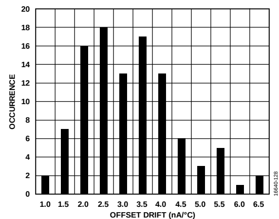
Figure 28. Offset Error Drift Distribution Histogram (Current Input)
