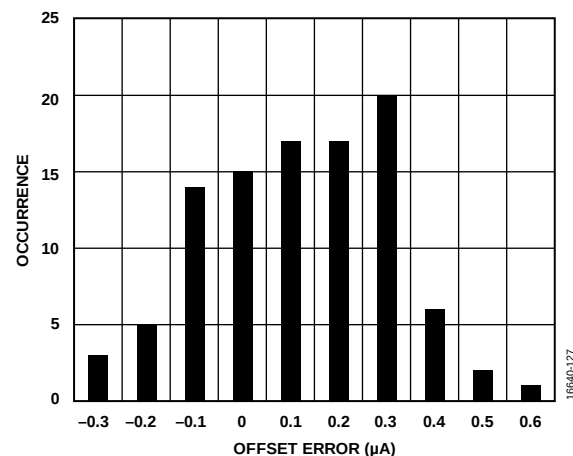
Figure 27. Offset Error Distribution Histogram (Current Input)
