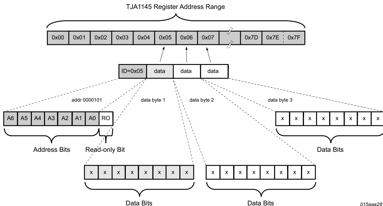
Fig 11. SPI data structure for a write operation (16-, 24- or 32-bit)
