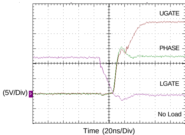
Dead Time
