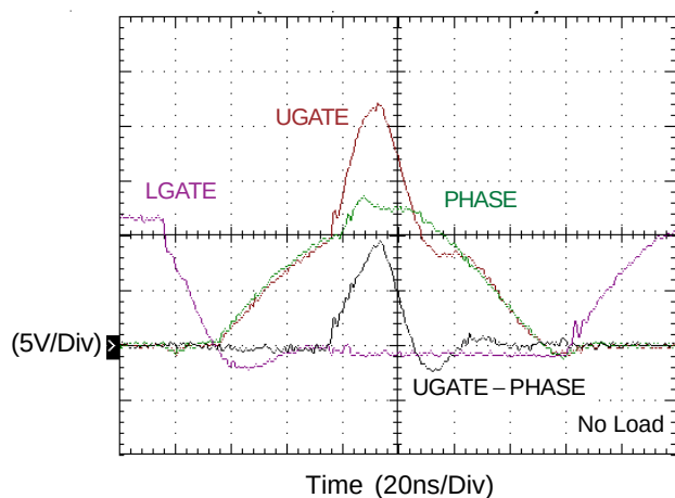
Short Pulse
