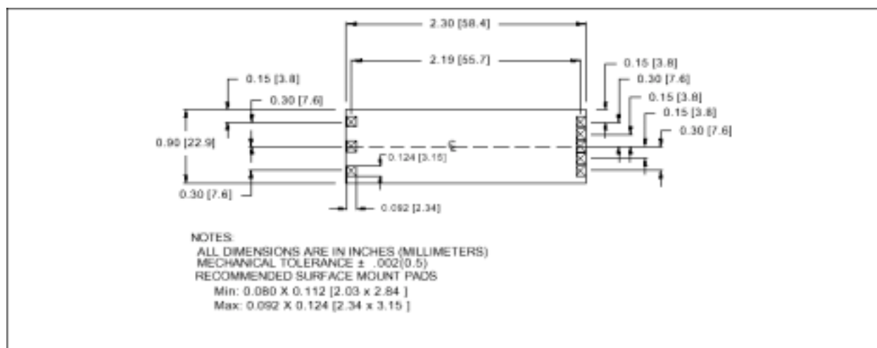
Figure 15. Recommended Pad layout for SMT (Suffix "S") version.
