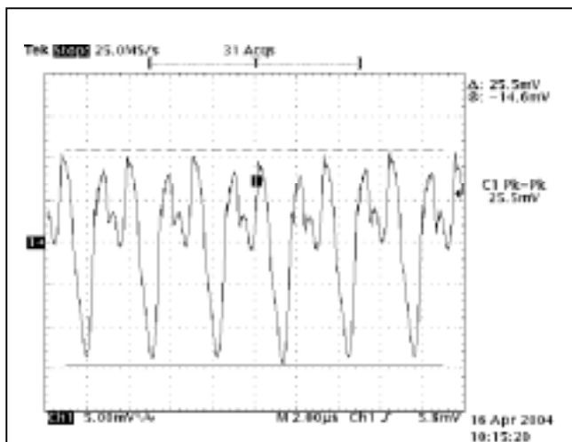
Figure 8. Output Ripple Waveform at V_{IN} = 24Vdc, I_O = Full Load, T_A = 25°C.
