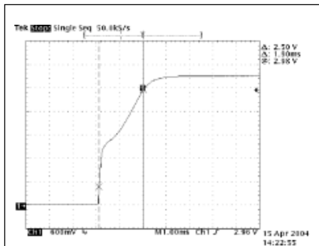
Figure 7. Output Turn On Response Time at V_{IN} = 24V, I_O = Full Load T_A = 25°C.
