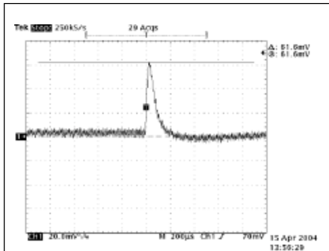
Figure 9. Output Transient Response at T_A = 25^\circ\text{C} ; Peak Deviation (Hi - Lo).
