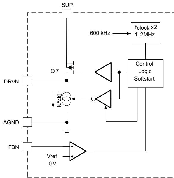
Figure 18. Negative Charge Pump Block TPS65165
