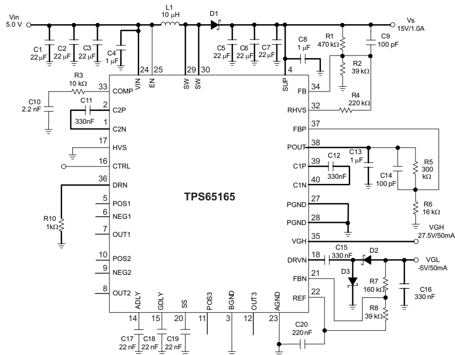
Figure 22. Layout Recommendation
