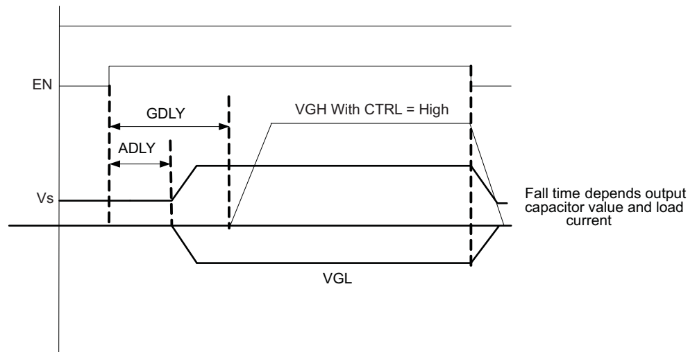
Figure 15. Power-On Sequencing
