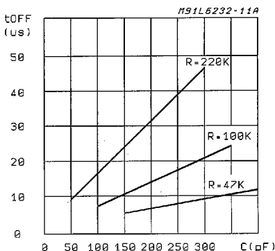
Figure 2: Typical toff vs. Capacity of C
