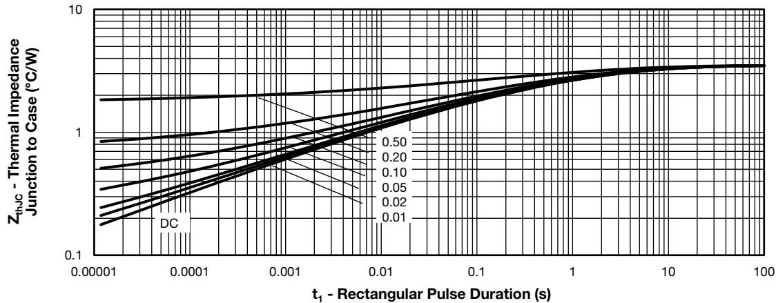
Fig. 6 - Transient Thermal Impedance, Junction to Case
