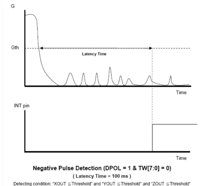
Figure 5. Freefall Detection in Pulse Mode
