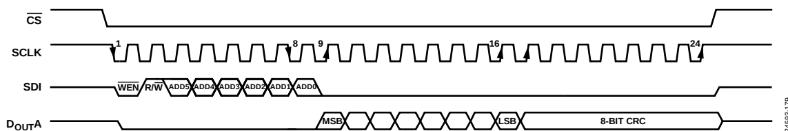
Figure 112. Reading Registers Through the SPI with CRC Enabled
