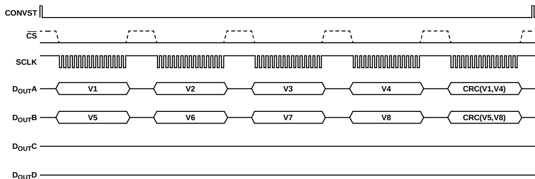
Figure 115. Serial Interface ADC Reading with CRC On, Two D OUTX Lines
