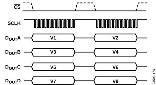
Figure 104. Serial Interface ADC Reading, Four DOUTX Lines
