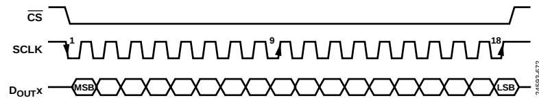
Figure 107. Serial Interface Data Read Back (One Channel)
