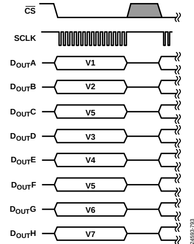
Figure 105. Serial Interface ADC Reading, Eight DOUTX Lines
