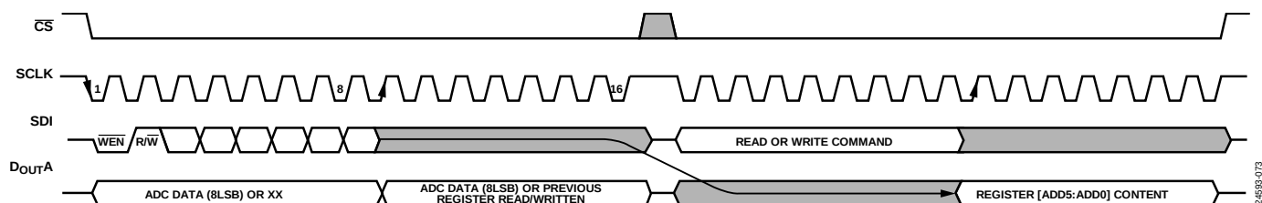
Figure 109. Serial Interface Read Command, First Frame Provides the Address, Second Frame Provides the Register Content
