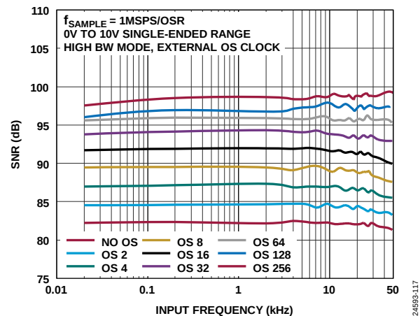
Figure 26. SNR vs. Input Frequency for Different OSR Values, 0\text{ V to } 10\text{ V} Single-Ended Range, High Bandwidth Mode, External Oversampling Clock
