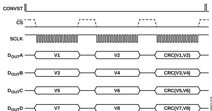
Figure 114. Serial Interface ADC Reading with CRC On, Four D OUTX Lines
