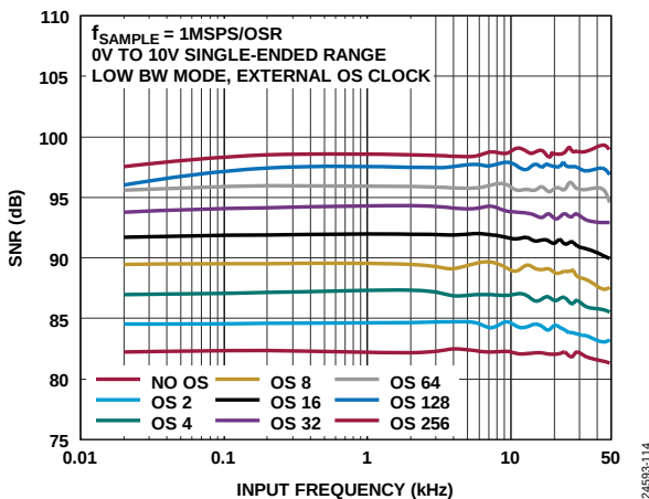
Figure 23. SNR vs. Input Frequency for Different OSR Values, 0\text{ V to } 10\text{ V} Single-Ended Range, Low Bandwidth Mode, External Oversampling Clock
