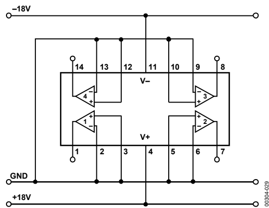
Figure 30. Burn-In Circuit
