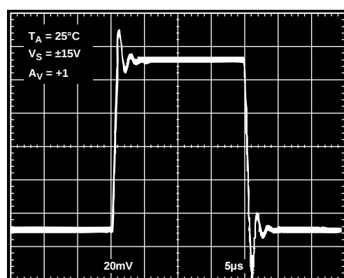
Figure 26. Small Signal Transient Response
