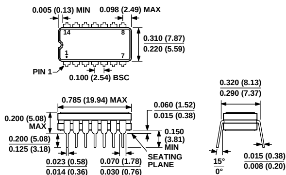
Figure 35. 14-Lead Ceramic Dual In-Line Package [CERDIP]
