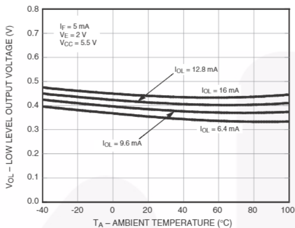
Figure 3. Low Level Output Voltage vs. Ambient Temperature
