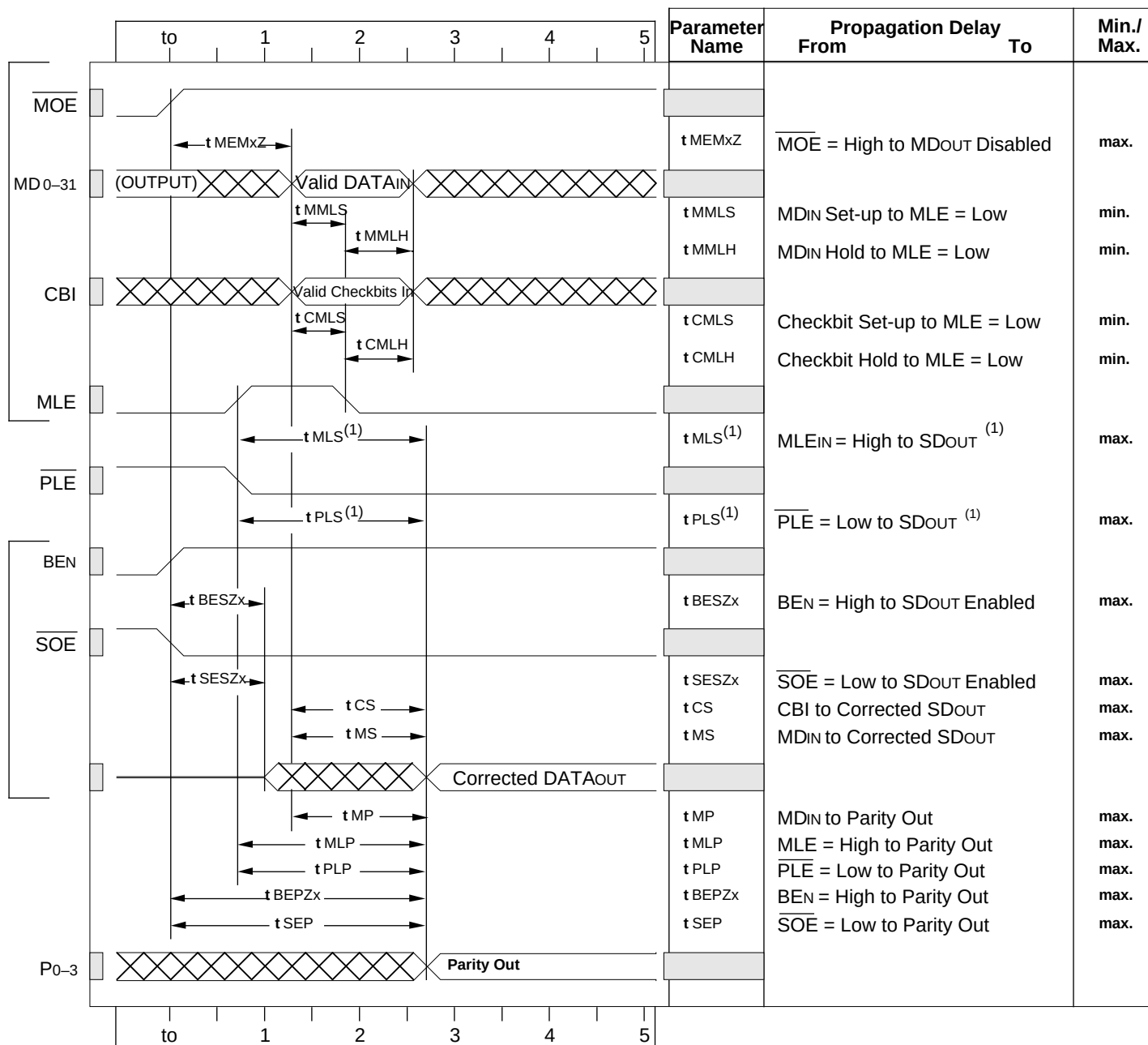
Figure 9. 32-Bit Correct Timing
