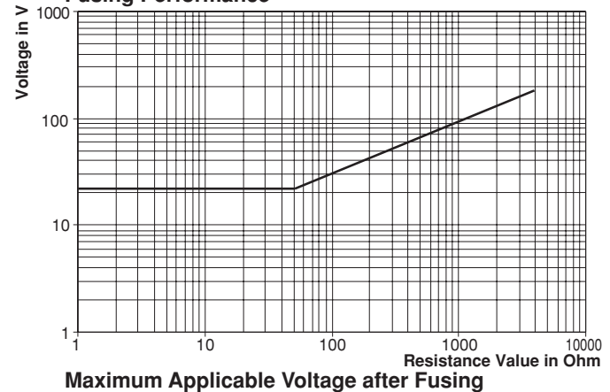
Fusing Performance
