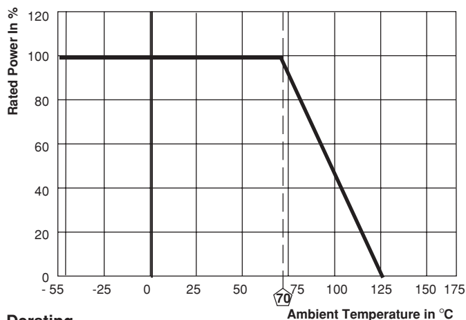
Derating
