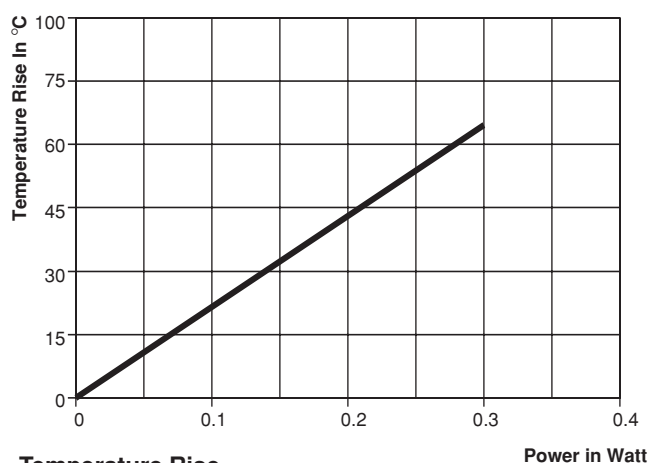
Temperature Rise
