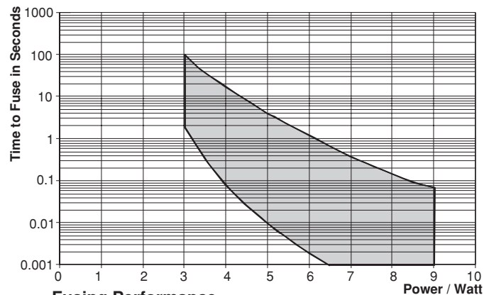
Fusing Performance
