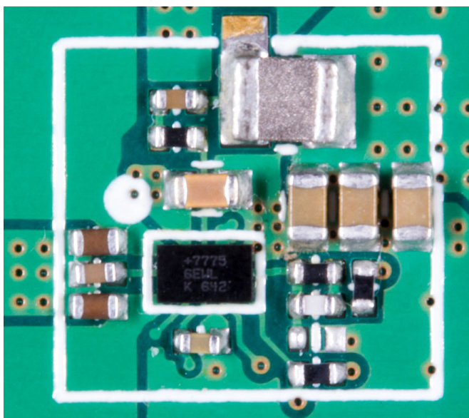
Figure 3. MAX77756 EV Kit PCB—Top View Solution Area
