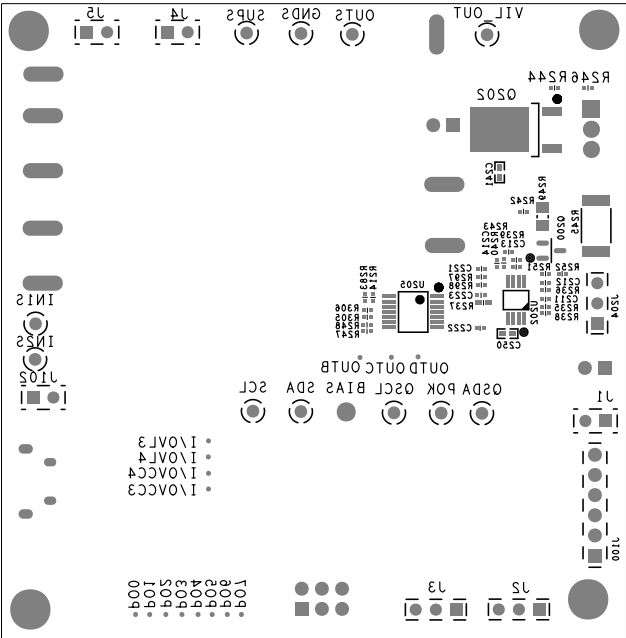
MAX77756 EV Kit Component Placement Guide—Bottom Silkscreen
