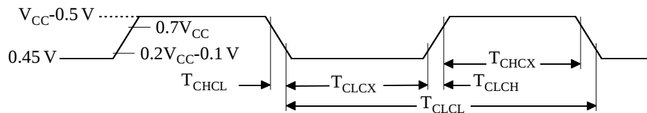
Figure 30. External Clock Drive Waveforms
