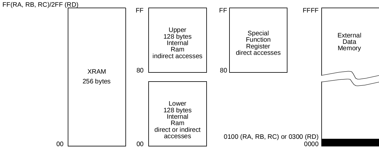
Figure 4. Internal and External Data Memory Address
