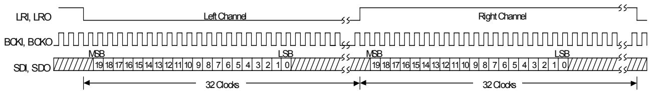
Fig. 4-7 I²S Data Format 64Fs, 20bit Data
