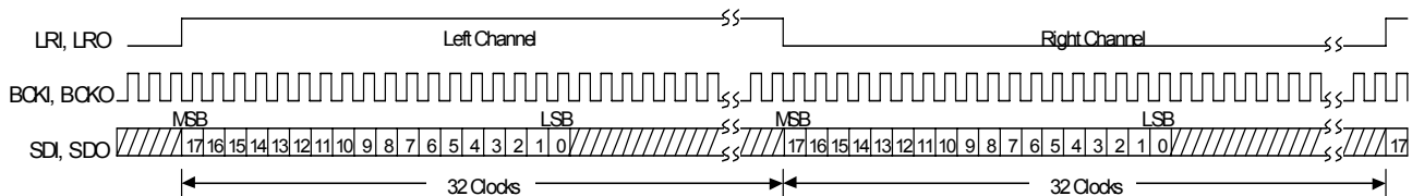
Fig. 4-8 Left-Justified Data Format 64Fs, 18bit Data
