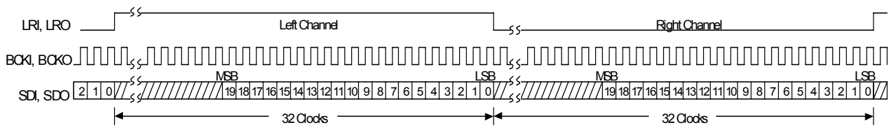
Fig. 4-6 Right-Justified Data Format 64Fs, 20bit Data
