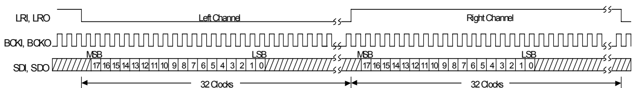
Fig. 4-10 I²S Data Format 64Fs, 18bit Data
