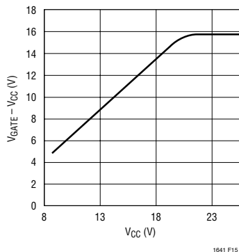
Figure 15. Gate Drive vs Supply Voltage
